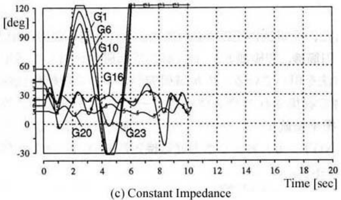
Fig.5.7 Additional Case (the load characteristic is changed) 1cct. 3LG-O at Point C (Daytime Condition)
