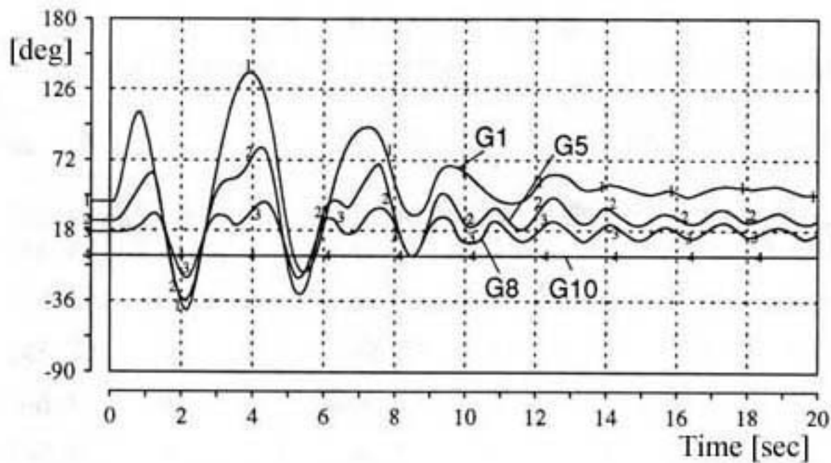
(a) NLT = 2 (Constant Current) (Base Case)
