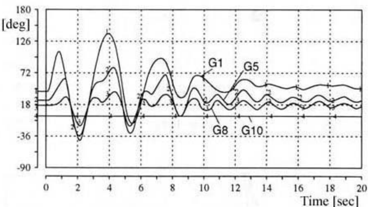
(b) NLT = 107 (Constant Current, refer Fig. 1.5)
