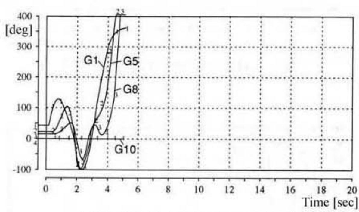
(a) Generator Internal Angle (G10 Base)
