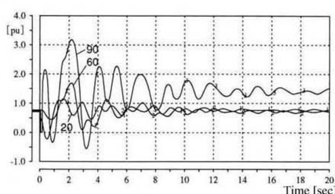
(c) Line Active Power Flow (1,000 MVA Base)
