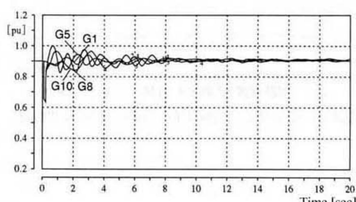
(b) Generator Active Power Output (Gen. Self Capacity Base)
