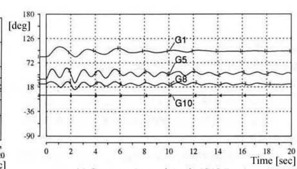
(a) Generator Internal Angle (G10 Base)
