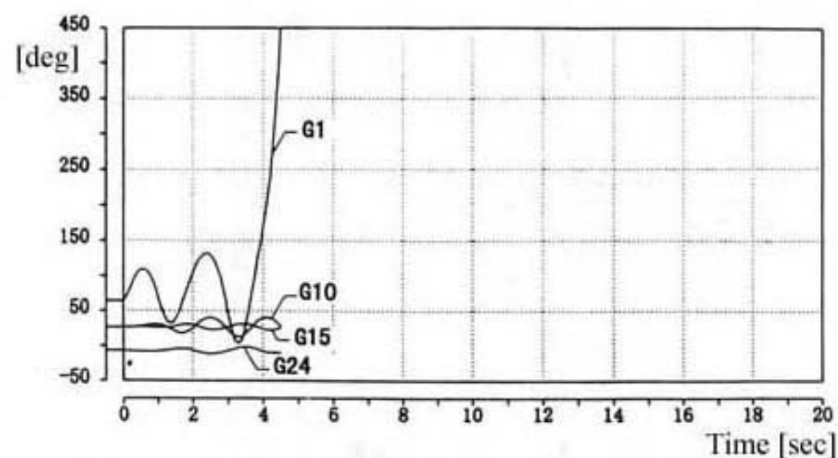
(b) The Excitation System of G1, G4 and G9 are changed to LAT = 2 (Thyristor Exciter Model)
