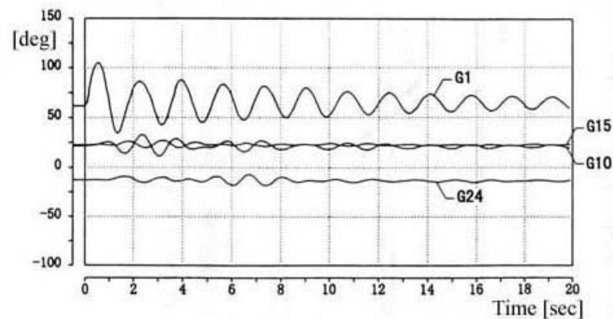
(c) The Excitation System of G1, G4 and G9 are changed to LAT = 102 (Thyristor Exciter + PSS)
