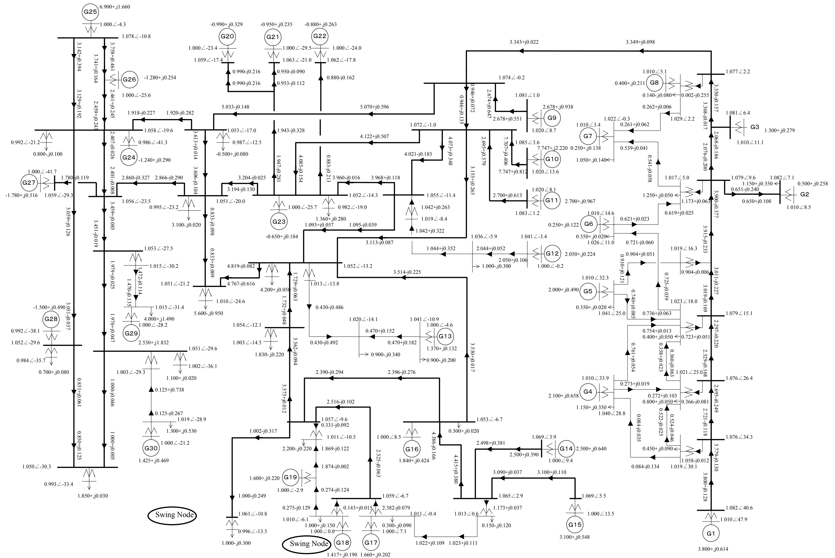
Fig.4.3(b) IEEJ EAST 30-machine System Model (Load Flow Map : Nighttime Condition)
