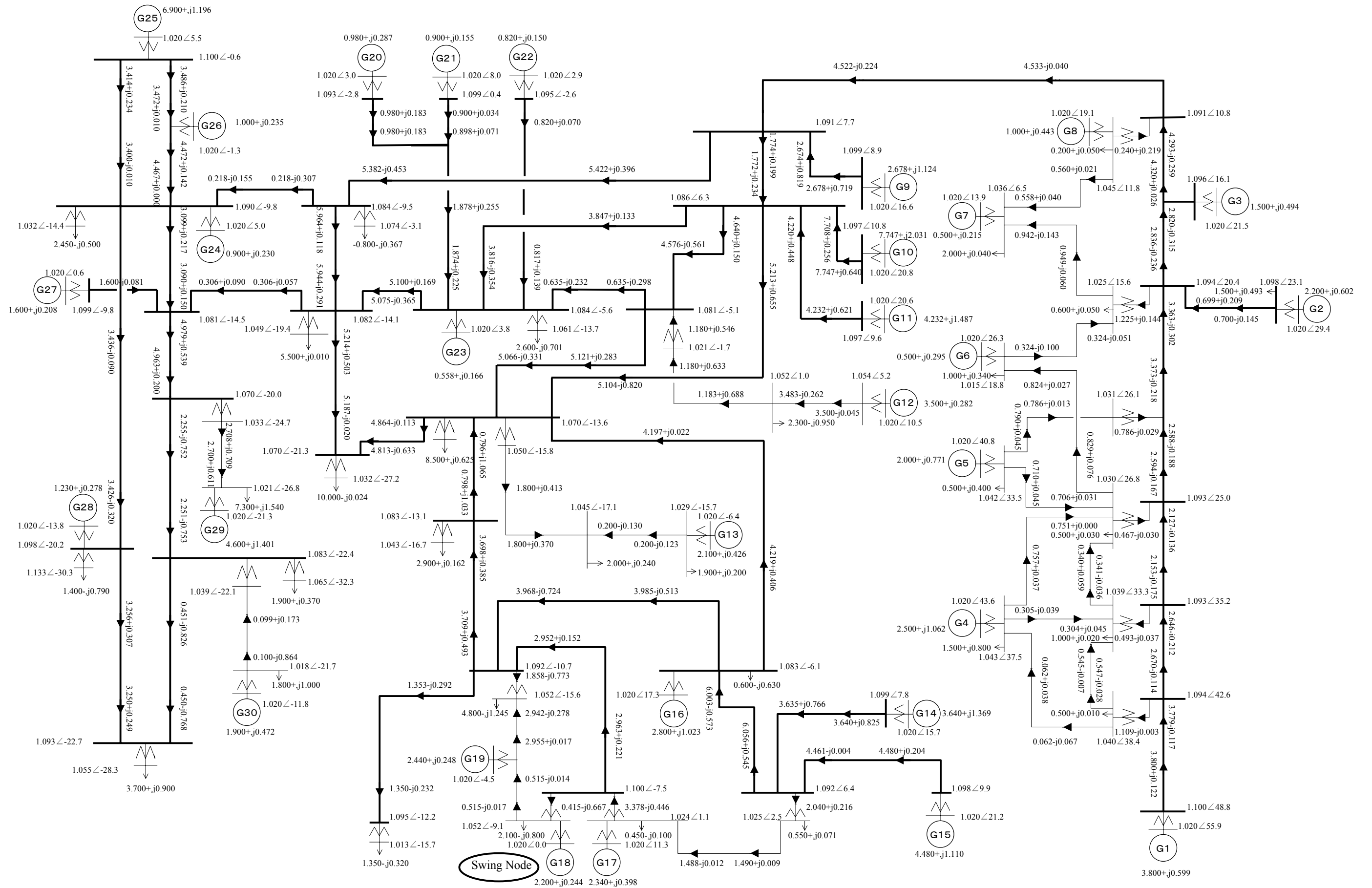
Fig.4.3(a) IEEJ EAST 30-machine System Model (Load Flow Map : Daytime Condition)
