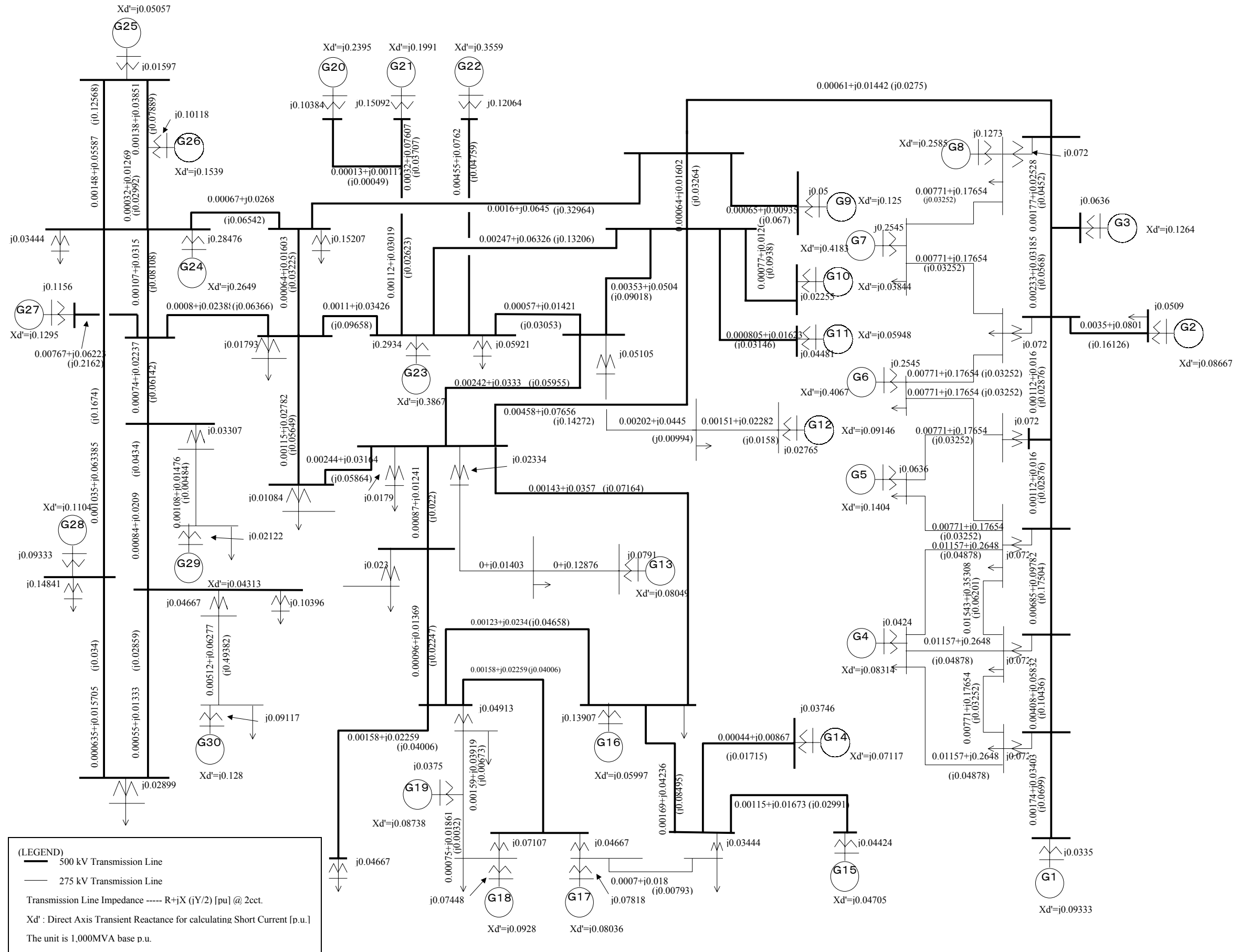
Fig.4.2 IEEJ EAST 30-machine System Model (Impedance Map)
