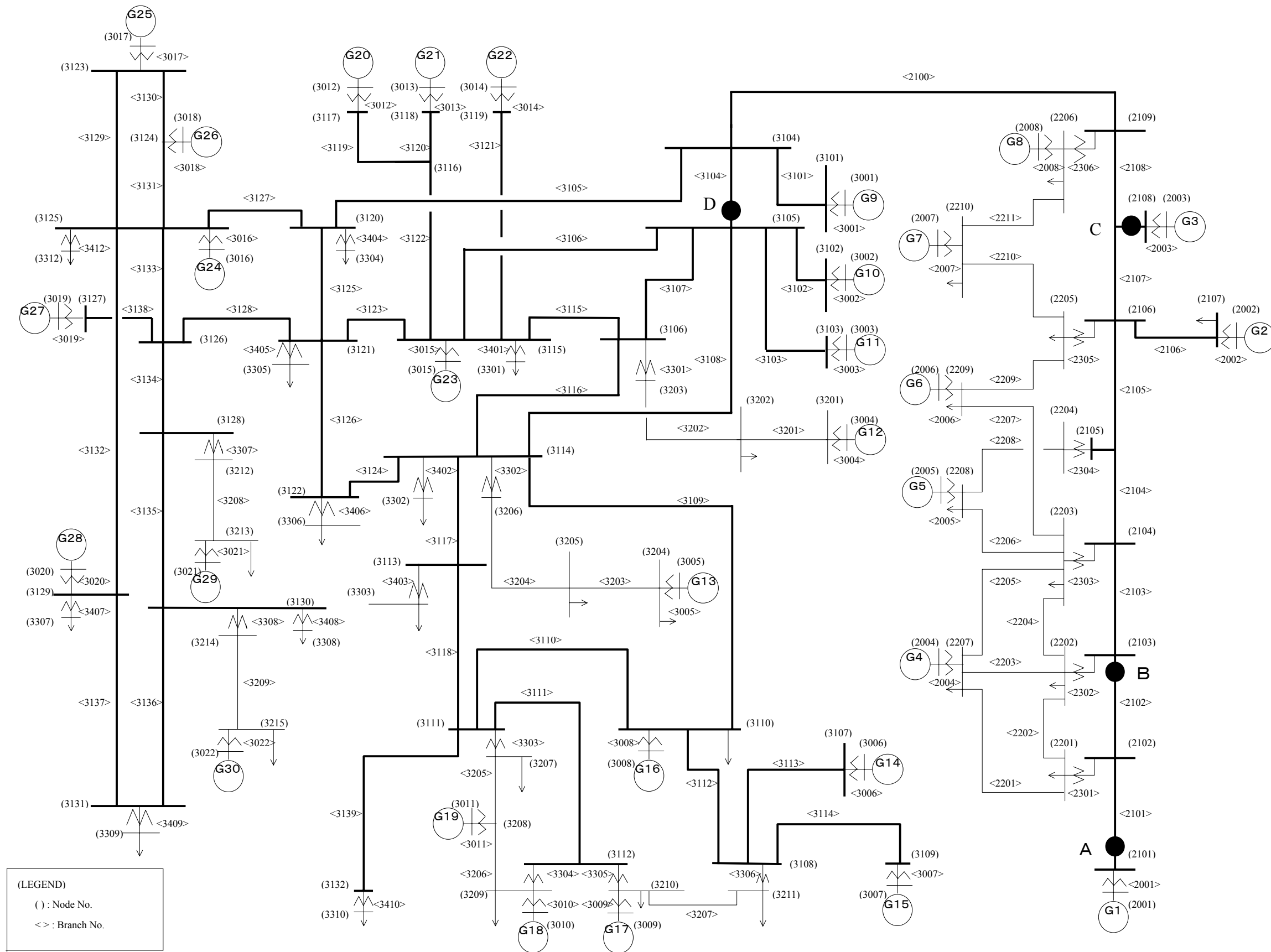
Fig.4.1 IEEJ EAST 30-machine System Model (Node No., Branch No., Disturbance Point)
